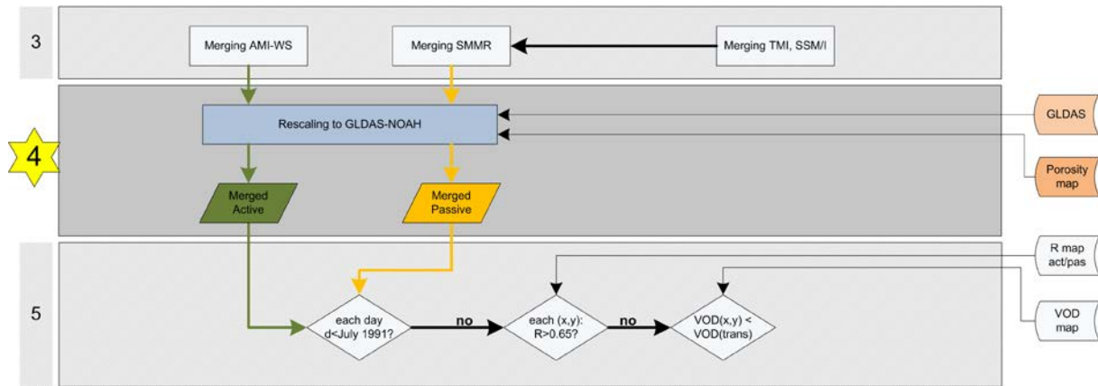
Figure 5-5: Processing step 4: Rescaling to GLDAS climatology
