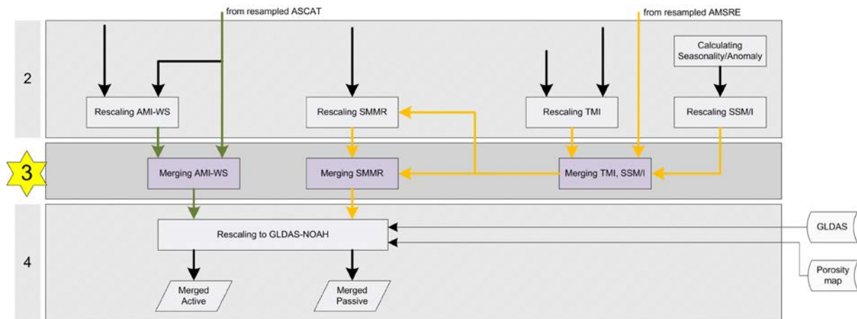
Figure 5-4 Processing step 3: Active Merging and Passive Merging
