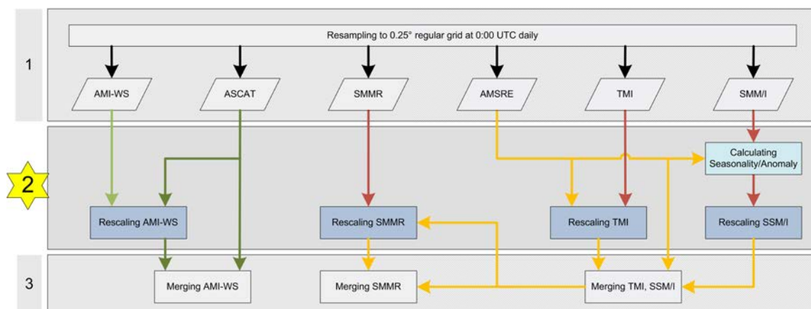
Figure 5-3: Processing step 2: Rescaling
