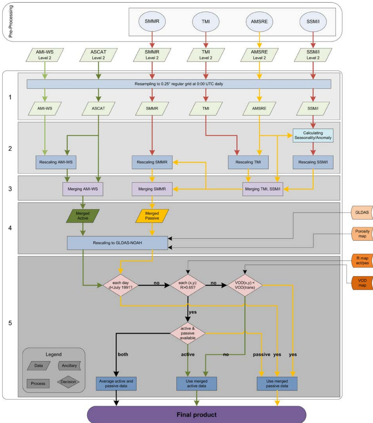
Figure 5-1. An overview of processes in the ECV SSM product generation
