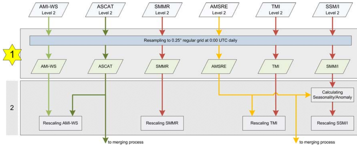
Figure 5-2: Processing step 1: Resampling of the input data sets
